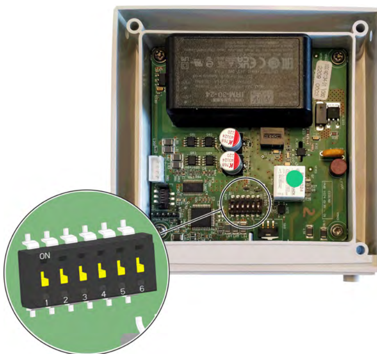
Fig. 19: Switch bar on the board
