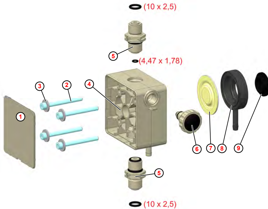
Abb. 29: Pumpenkopf 11 l/h
