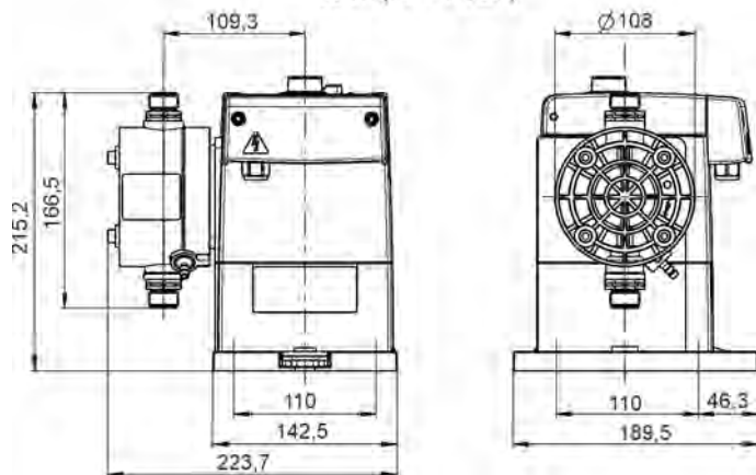
Fig. 36: Dimensions 30 l/h
