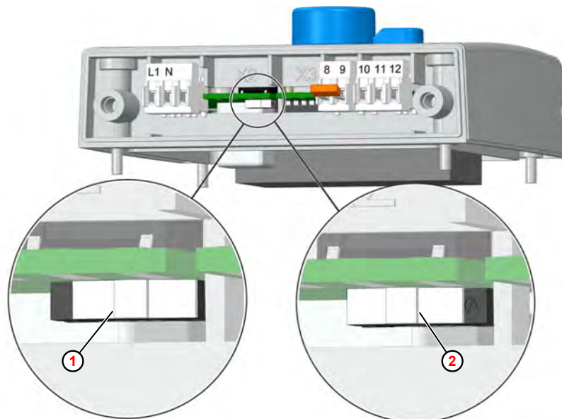
Fig. 14: Activating AutoStart
