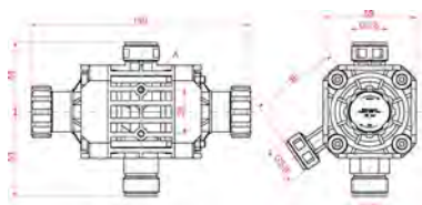
Fig. 9 : Dimensions, raccords
