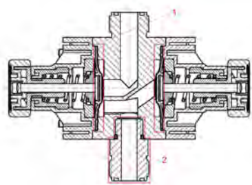
Fig. 7: Replacement parts
