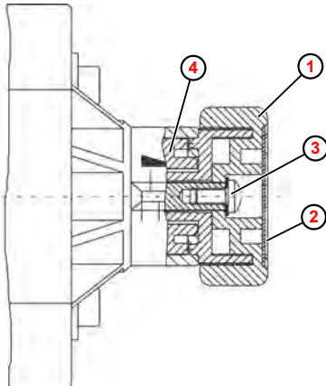
Fig. 5: Setting the overpressure (overpressure function)
