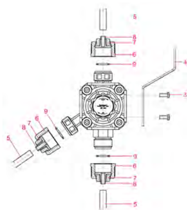
Fig. 2: Installing the MFV II-III, model 3
