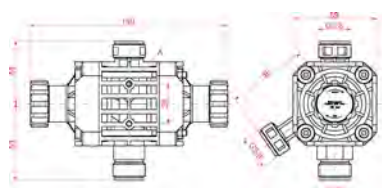
Fig. 9: Dimensions, connections
