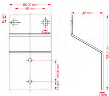
Fig. 8: Accessories
