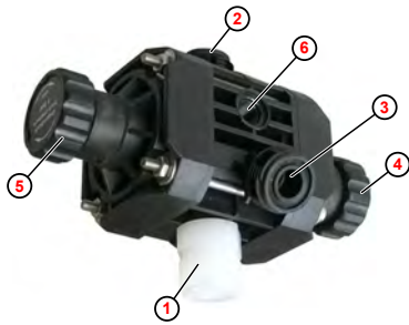
Fig. 1: Structure of the MFV II-III, model 3
