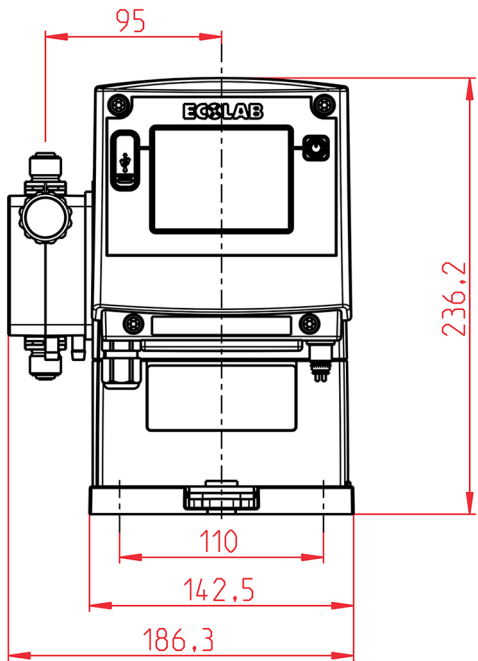
EcoAdd 5/11 l/h
