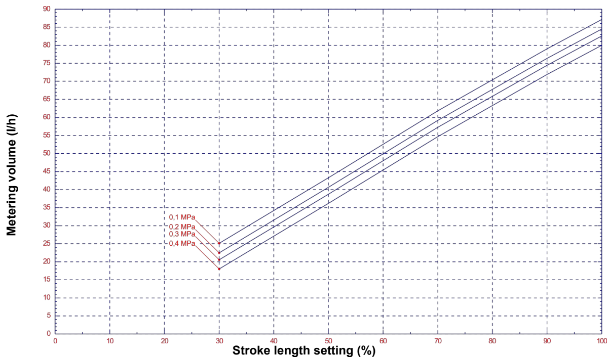
Fig. 14.14 Delivery capacity type 00800 / 0.4 MPa (4 bar)
