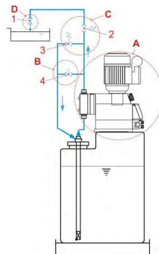
Fig. 7.1 Device installation Hydraulic installation Installation examples 1
