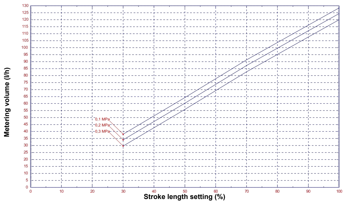
Fig. 14.15 Delivery capacity type 01200 / 0.3 MPa (3 bar)
