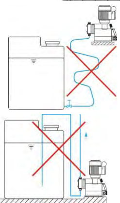
Fig. 7.7 Device installation: Hydraulic installation Installation examples 7
