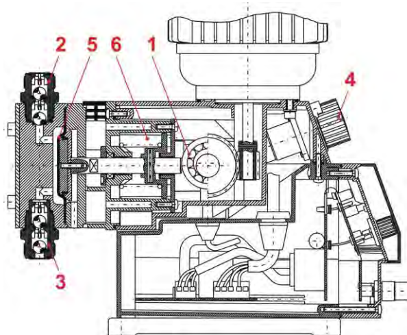
Fig. 4.1 Mechanical functions
