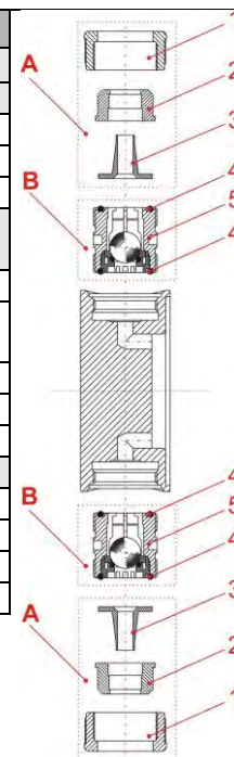
Fig. 11.1 Replacing the suction / pressure valve, type 00800 - 01200
