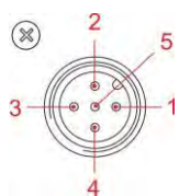
Fig. 8.6 Connector assignments of slot VII (5-terminal), input for batch pulse and metering lock
