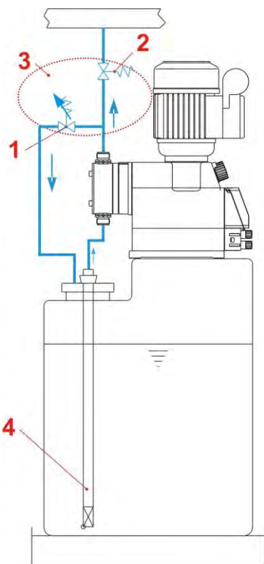
Fig. 6.1 Mounting diagram
