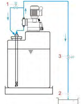
Fig. 7.5 Device installation: Hydraulic installation Installation examples 5
