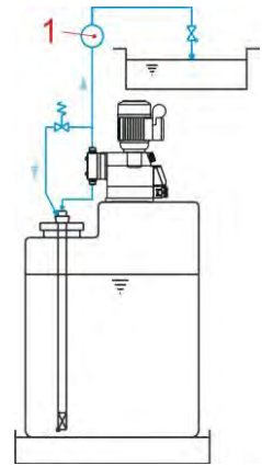
Fig. 7.10 Device installation: Hydraulic installation Installation examples 10
