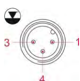
Fig. 7.14 Connector assignments of Slot I (3-terminal), Input for low level advance warning and empty report
