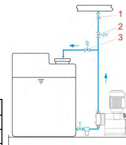
Fig. 7.2 Device installation : Hydraulic installation Installation examples 2
