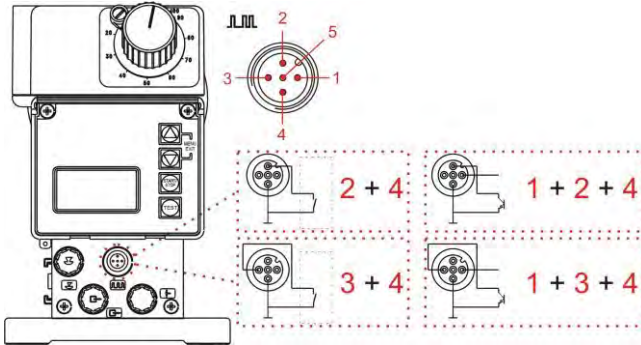
Fig. 7.21 Installing the metering monitoring
