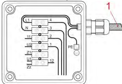
Fig. 7.12 Electrical installation: power supply
