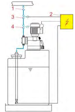
Fig. 7.3 Device installation: Hydraulic installation Installation examples 3
