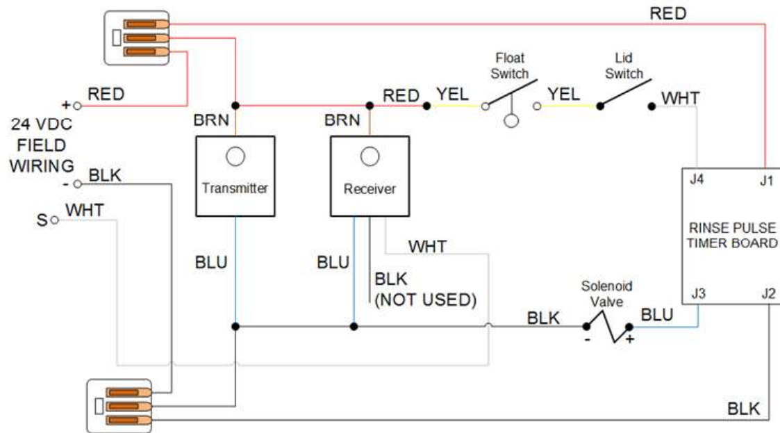
Fig. 2: Wiring diagram APEX Rinse Pulse Timer
