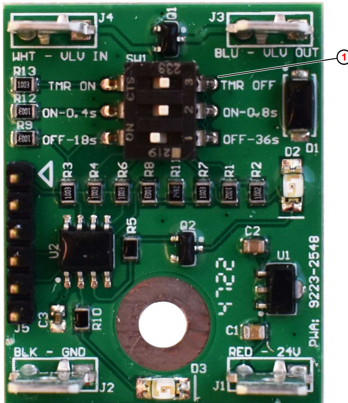
Fig. 4: Deactivation of the pulse timer
