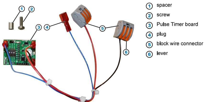
Fig. 1: Timer retrofit kit
