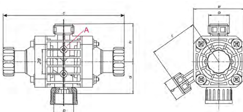
Fig. 10 : Dimensions, raccords
