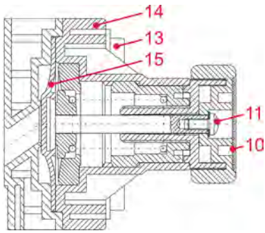
Fig. 7: Replacing the membranes
