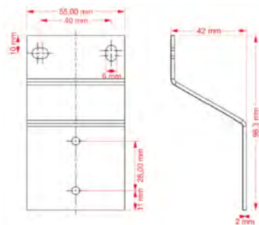
Fig. 9: Accessories
