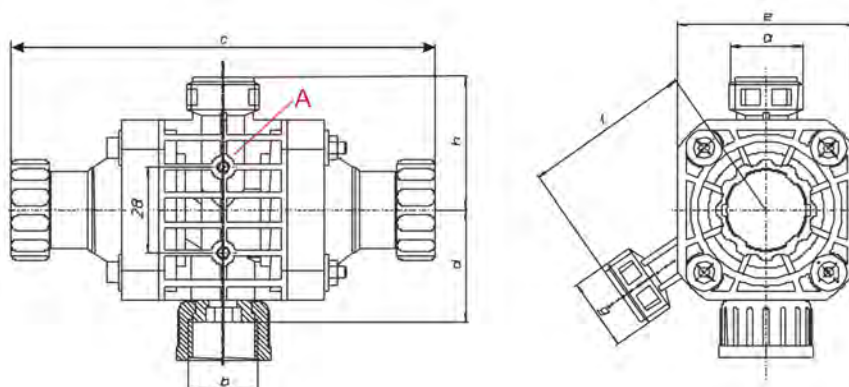
Fig. 10: Dimensions, connections
