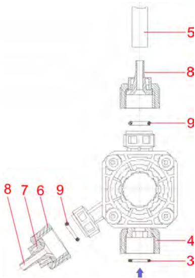
Fig. 2: Installing the MFV II-III, model 1, 2
