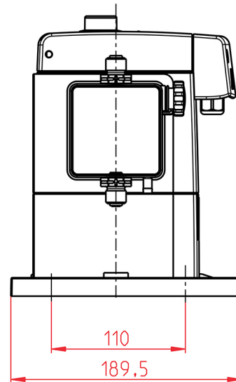
EcoPro/EcoEvo side view
