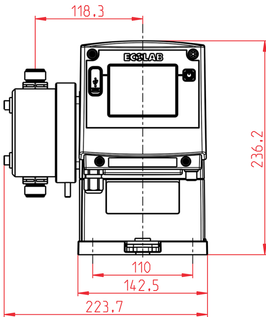
EcoAdd 30/50 l/h
